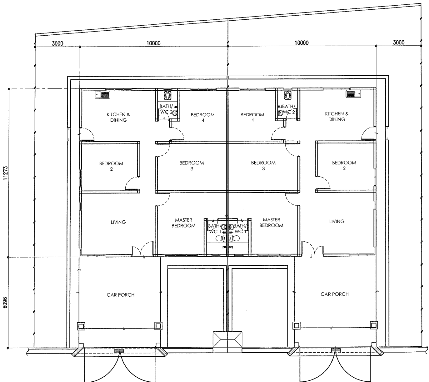
FLOOR PLAN
